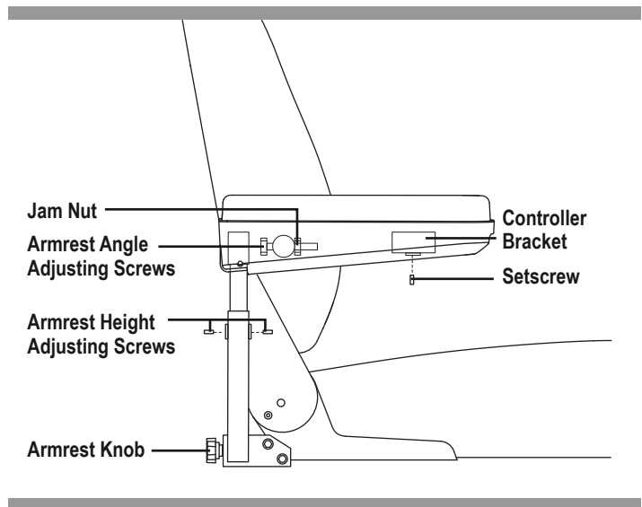
Figure 16. Seatback/Armrest Adjustment
